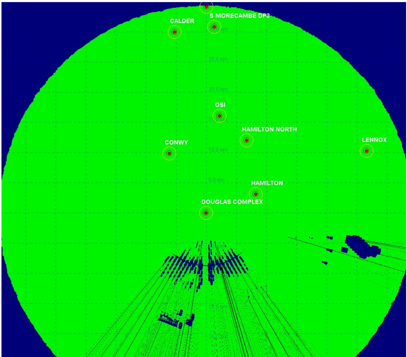
Figure 1.29: ENI Energy’s Douglas platform REWS detection plot showing loss regions for a 1,000 m 2 target.
