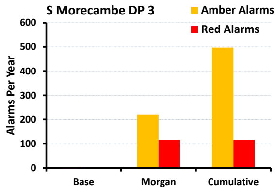
Figure 1.67: Modelled yearly alarm rates for the South Morecambe DP3 platform.
