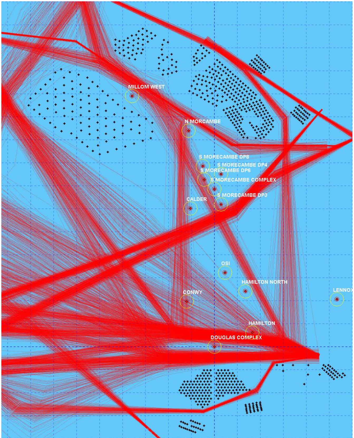
Figure 1.56: Modelled shipping routes post-construction of the Morgan Generation Assets.
