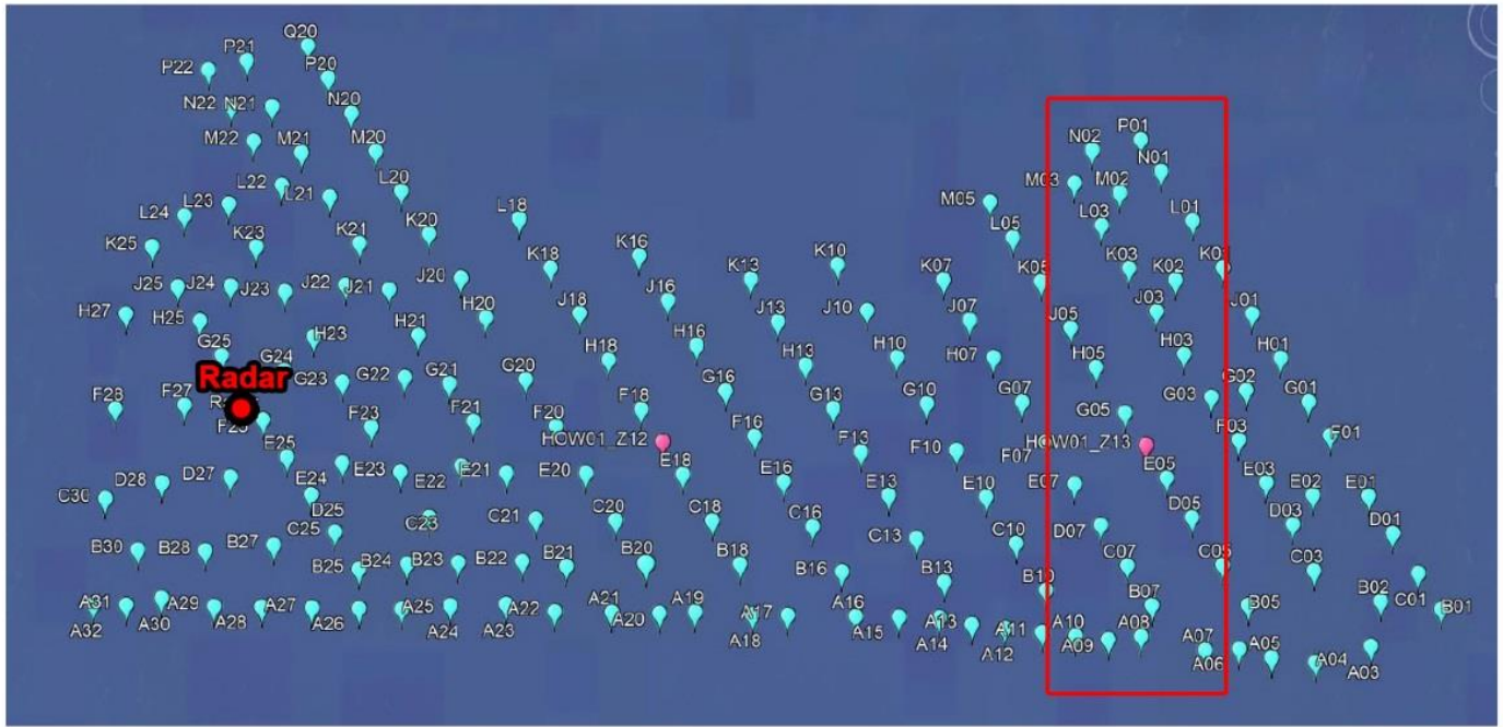
Figure 1.8: Wind turbine layout at Hornsea Project One array area and the location of the radar system used in the study. The red area denotes the region shown in Figure 1.9 (Terma, 2021).
