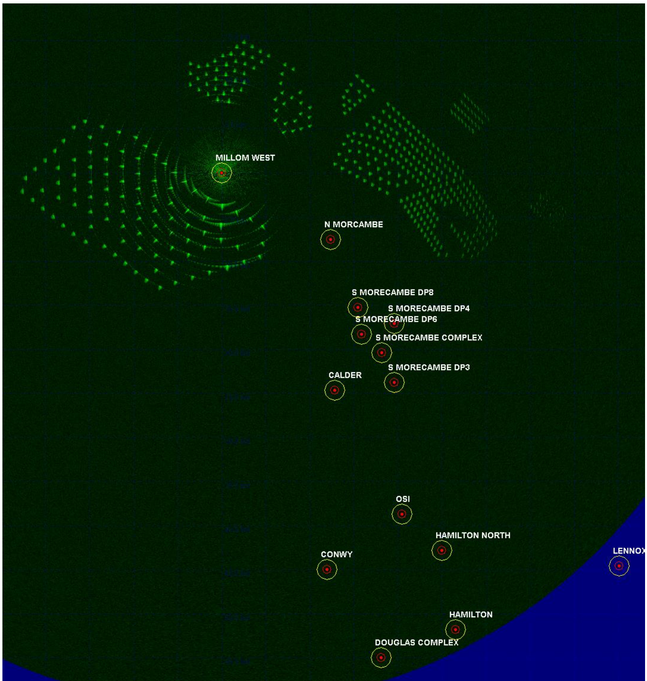
Figure 1.30: Harbour Energy’s Millom West platform REWS clutter map showing returns from the Morgan wind turbines and sea clutter.
