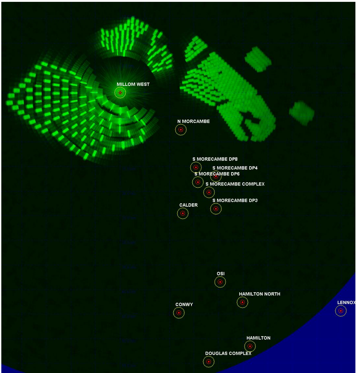
Figure 1.31: Harbour Energy’s Millom West platform REWS detection threshold over the Morgan Array Area.
