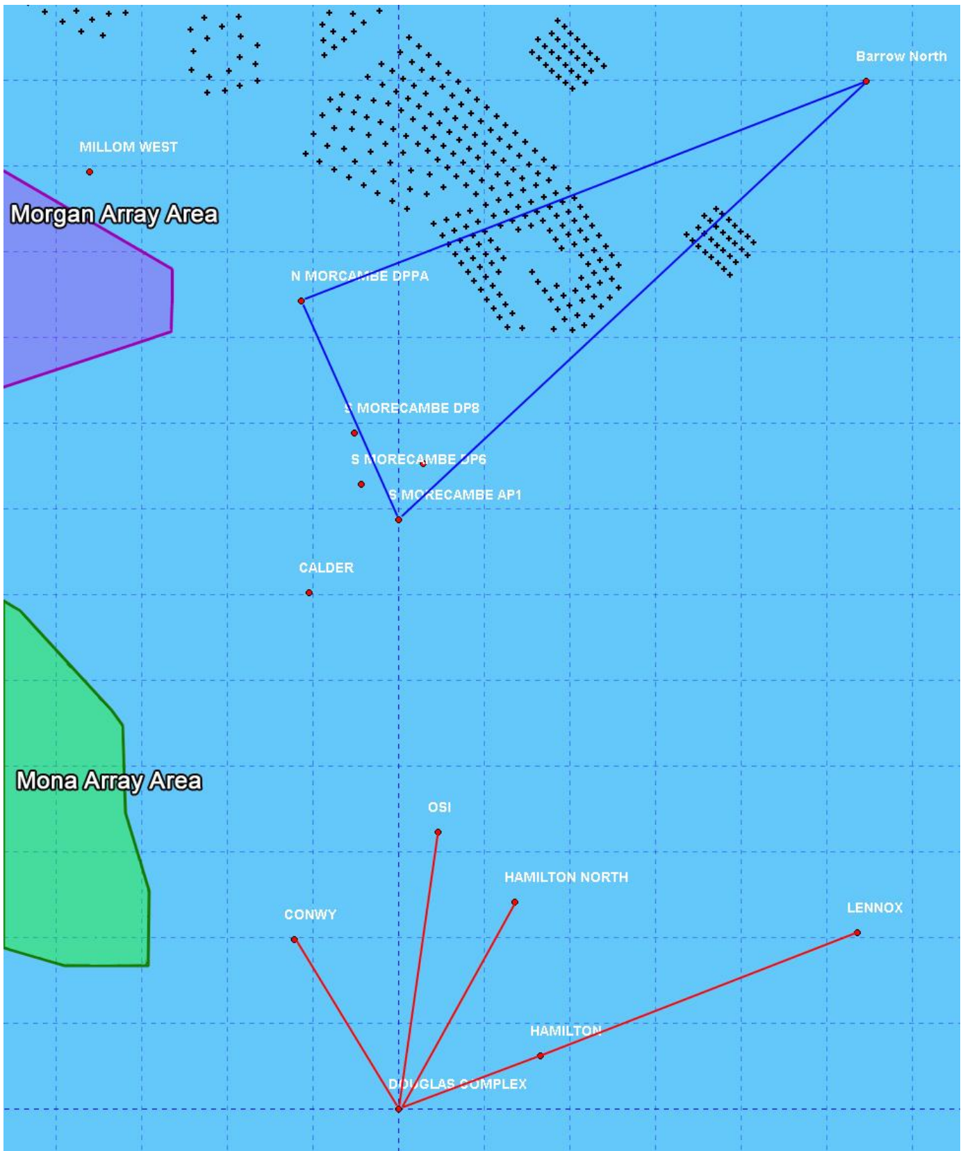
Figure 1.72: Layout of the modelled platforms and the communication links considered (red and blue lines indicate communication links).
