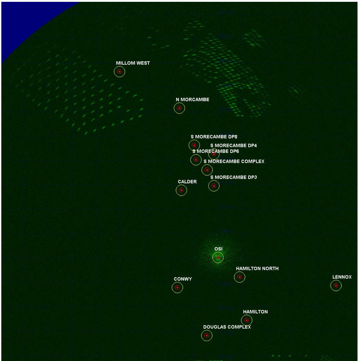
Figure 1.33: ENI Energy’s OSI REWS detection clutter map showing returns from the Morgan wind turbines and sea clutter.
