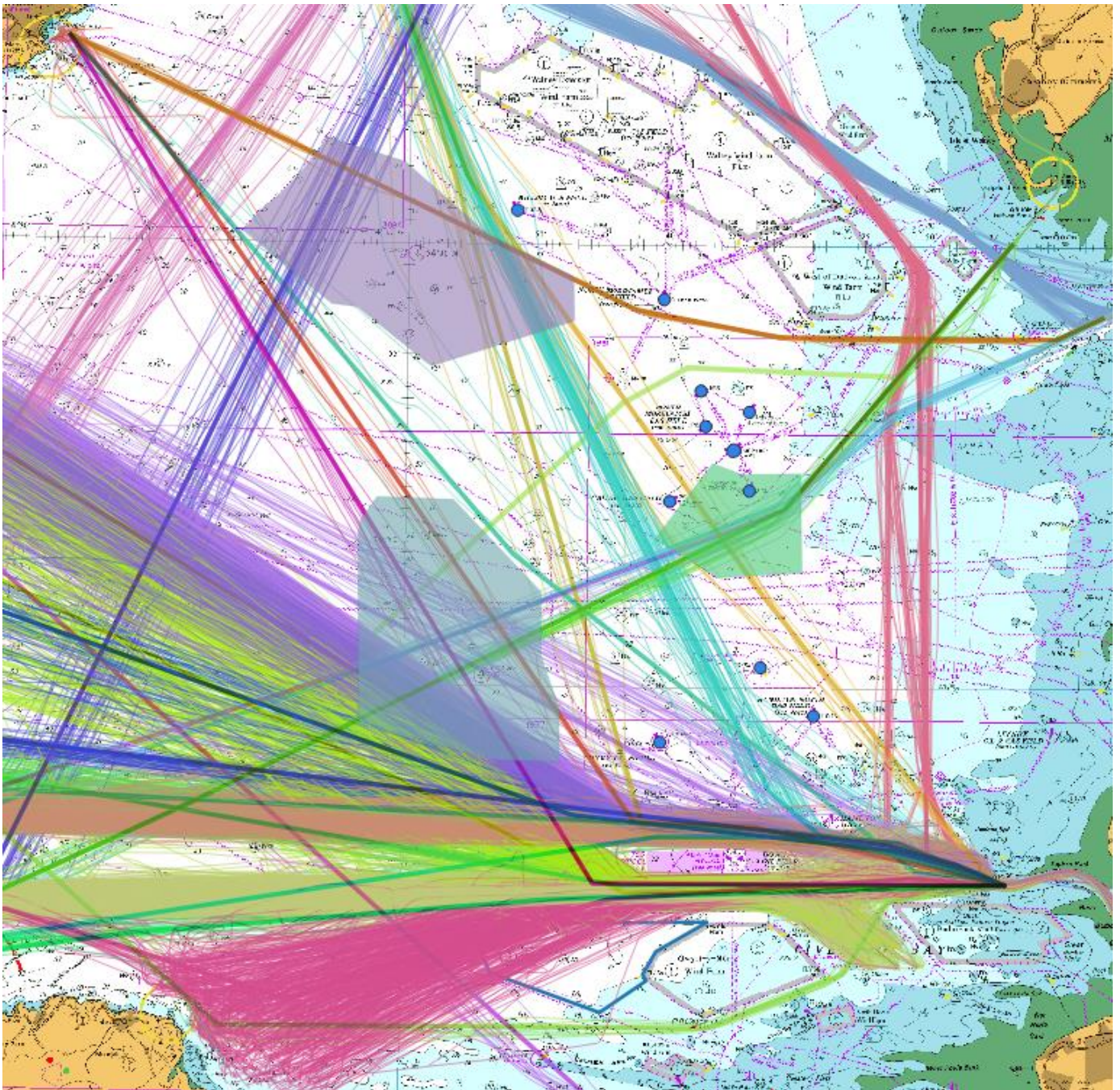
Figure 1.54: Existing commercial routes within and around the Morgan Array Area. 1
