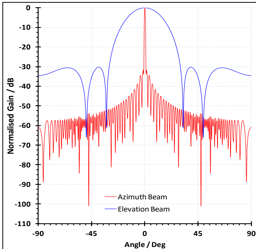
Figure 1.6: The radar antenna elevation and azimuth patterns.
