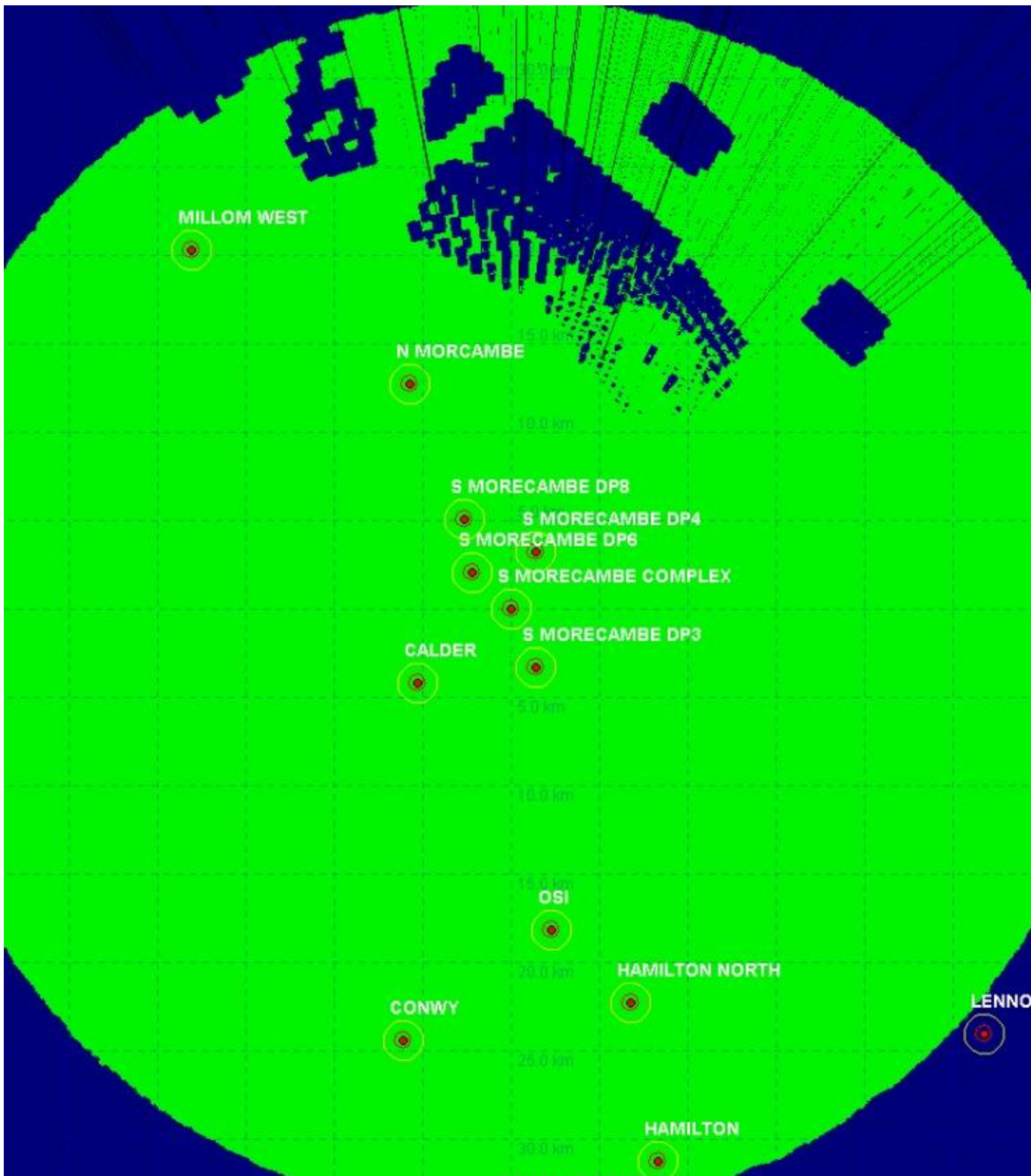
Figure 1.25: Spirit Energy’s South Morecambe AP1 platform REWS detection plot showing loss regions for a 1,000 m 2 target.
