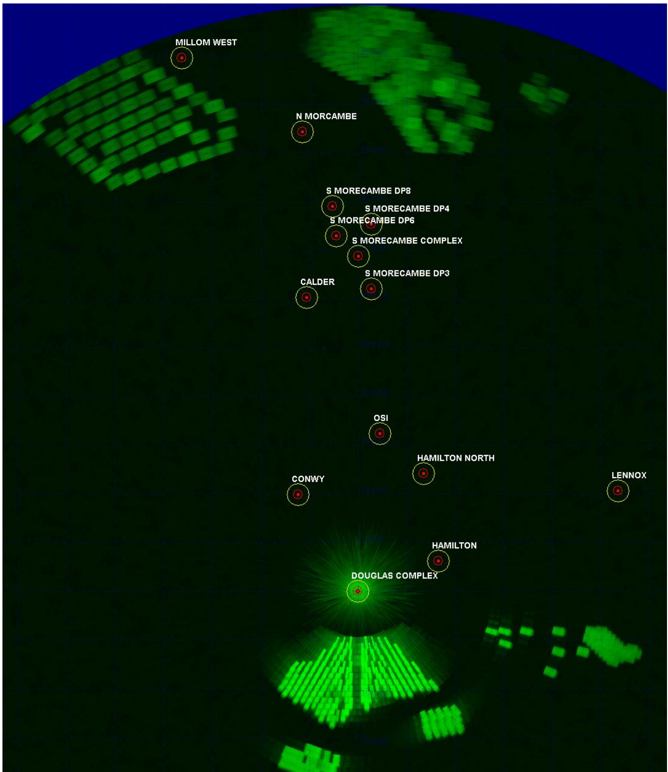
Figure 1.28: ENI Energy's Douglas platform REWS detection threshold over the Morgan Array Area.
