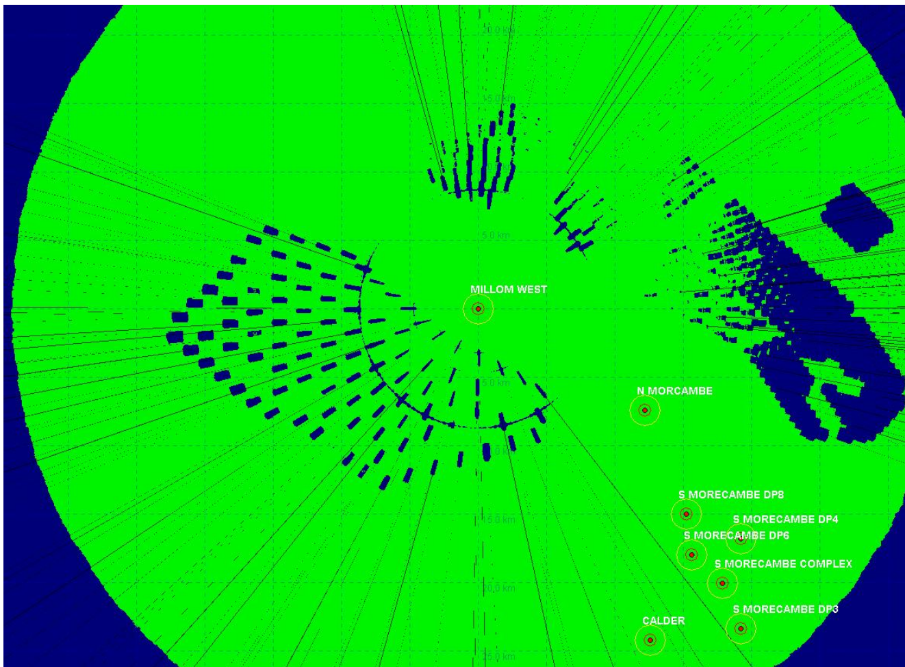
Figure 1.32: Harbour Energy’s Millom West platform REWS detection plot showing loss regions for a 1,000 m 2 target.
