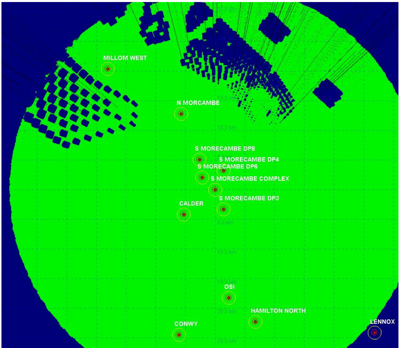
Figure 1.38: Spirit Energy’s South Morecambe AP1 platform REWS detection plot showing loss regions for a 1,000 m 2 target.
