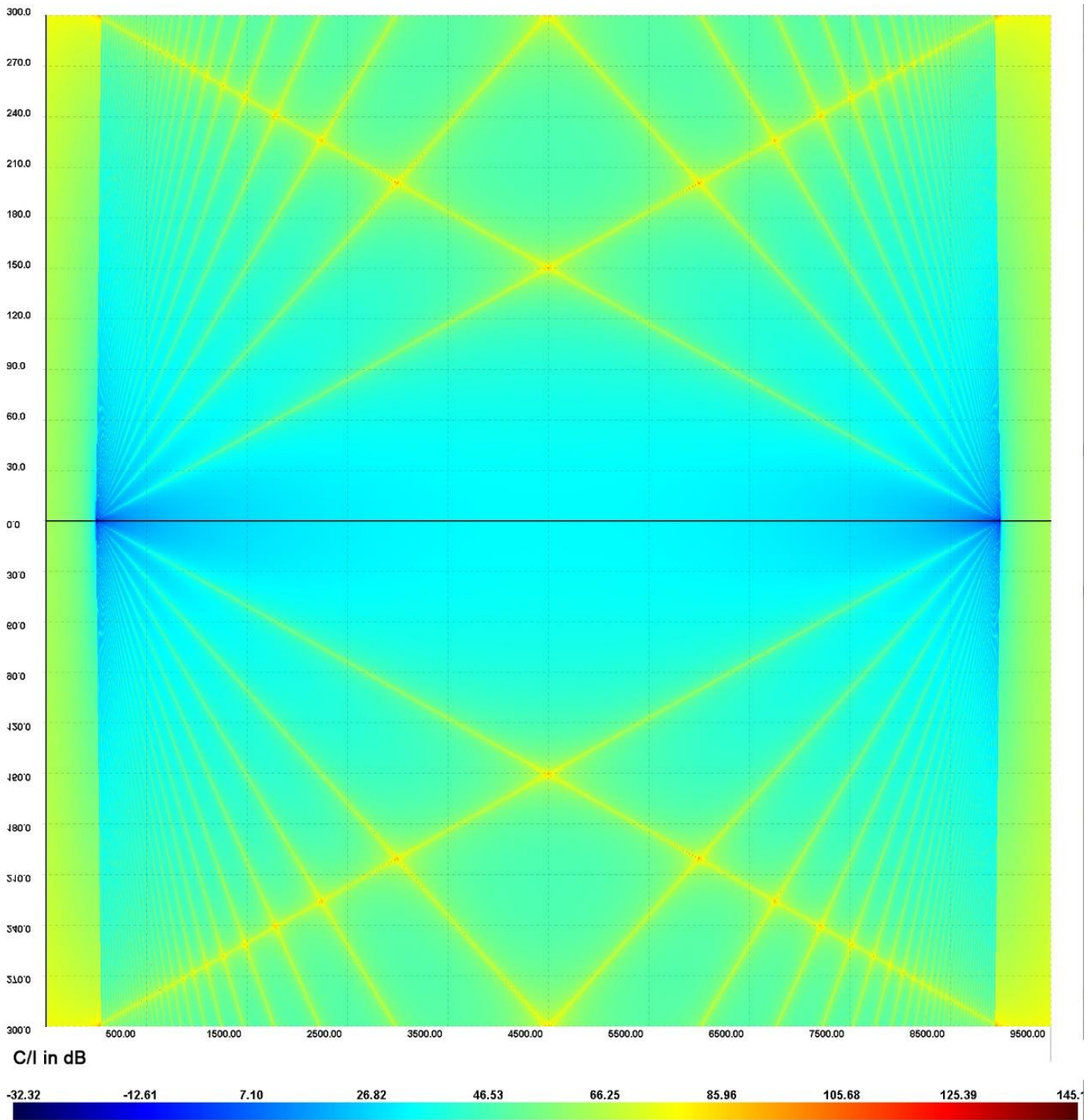
Figure 1.76: The signal to noise ratio around the Douglas – Hamilton link.
