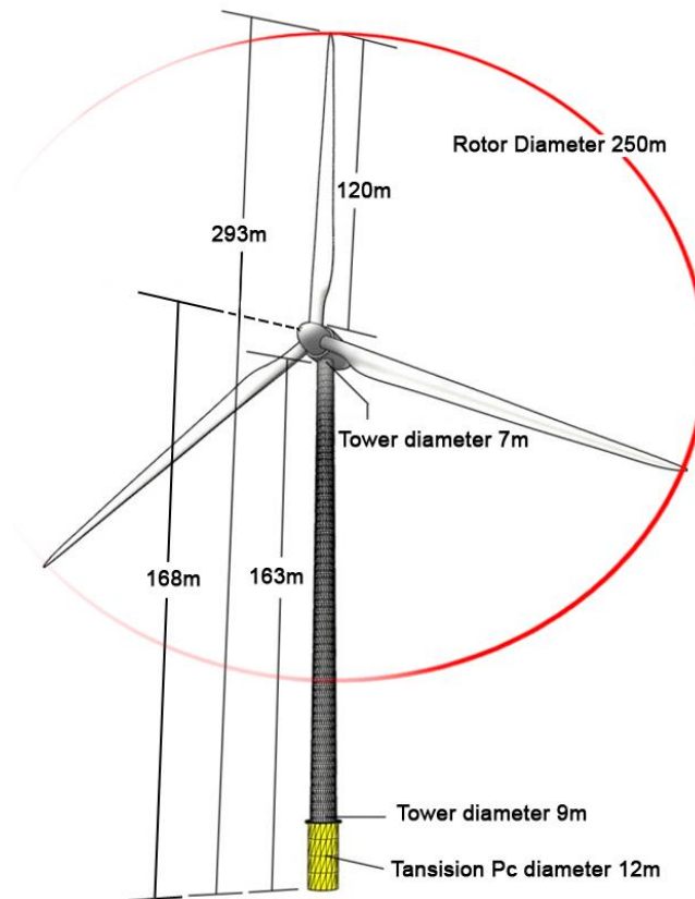
Figure 1.3: Modelled turbine geometry.
