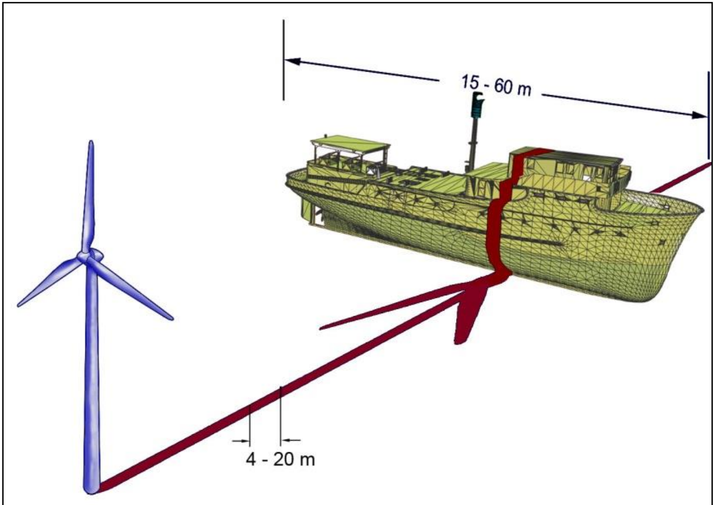
Figure 1.7: Optical blockage and partial shadowing.
