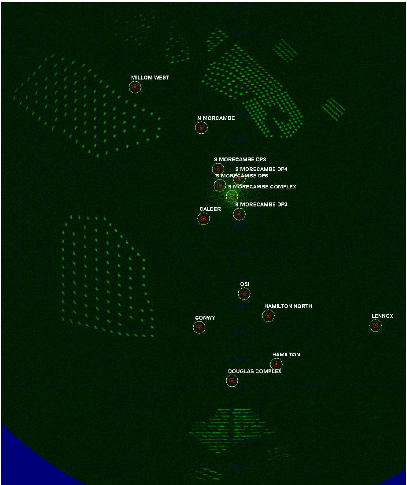
Figure 1.50: Spirit Energy’s South Morecambe AP1 platform REWS clutter map showing returns from the wind turbines and sea clutter.
