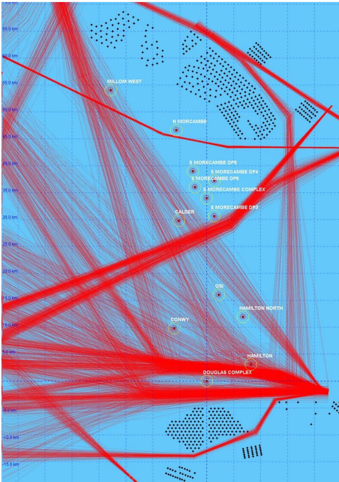
Figure 1.55: Modelled existing shipping routes (1,000 variations each route).
