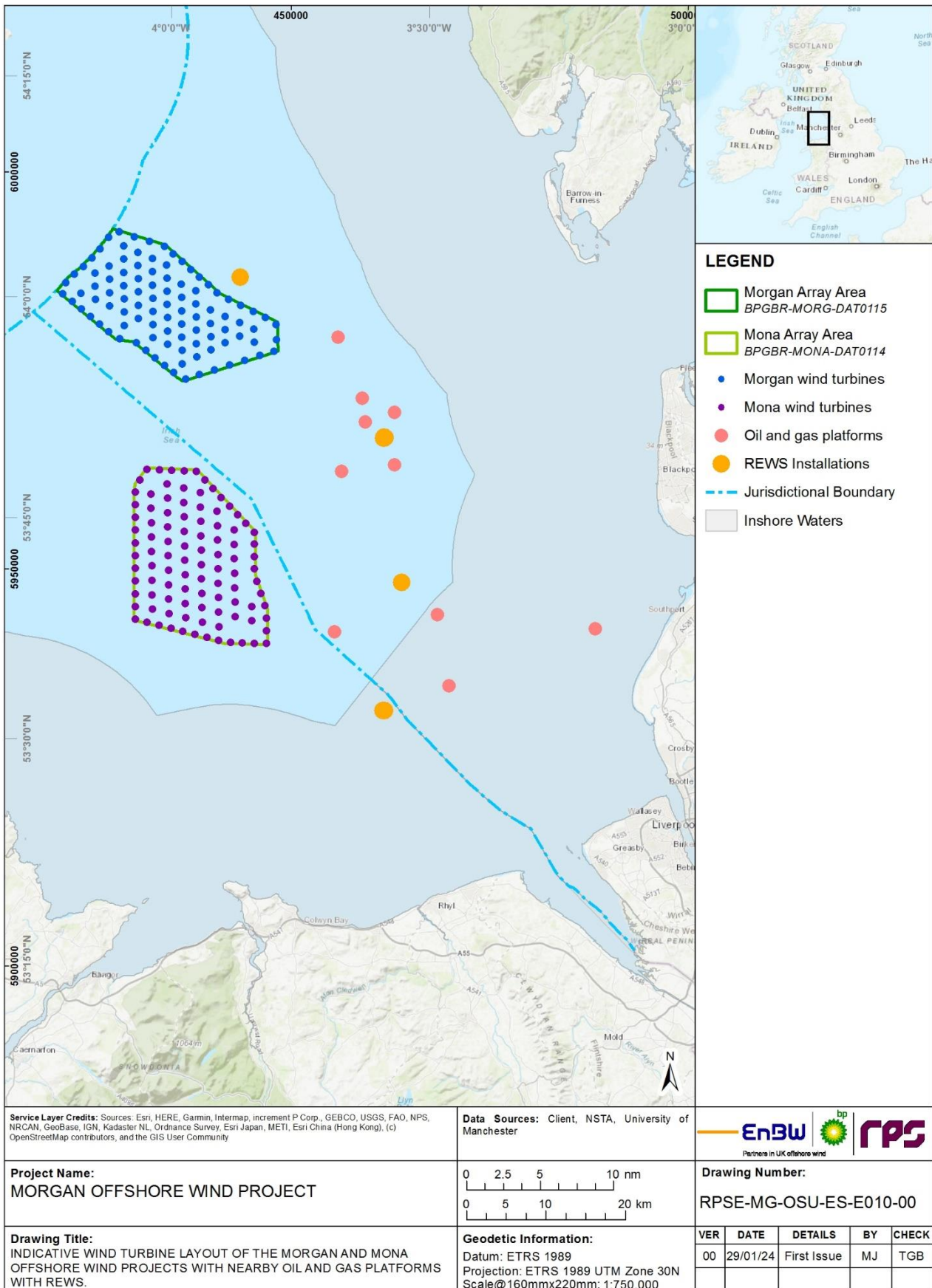
Figure 1.4: Indicative wind turbine layouts of the Morgan Generation Assets and Mona Offshore Wind Project with nearby oil and gas platforms with REWS.
