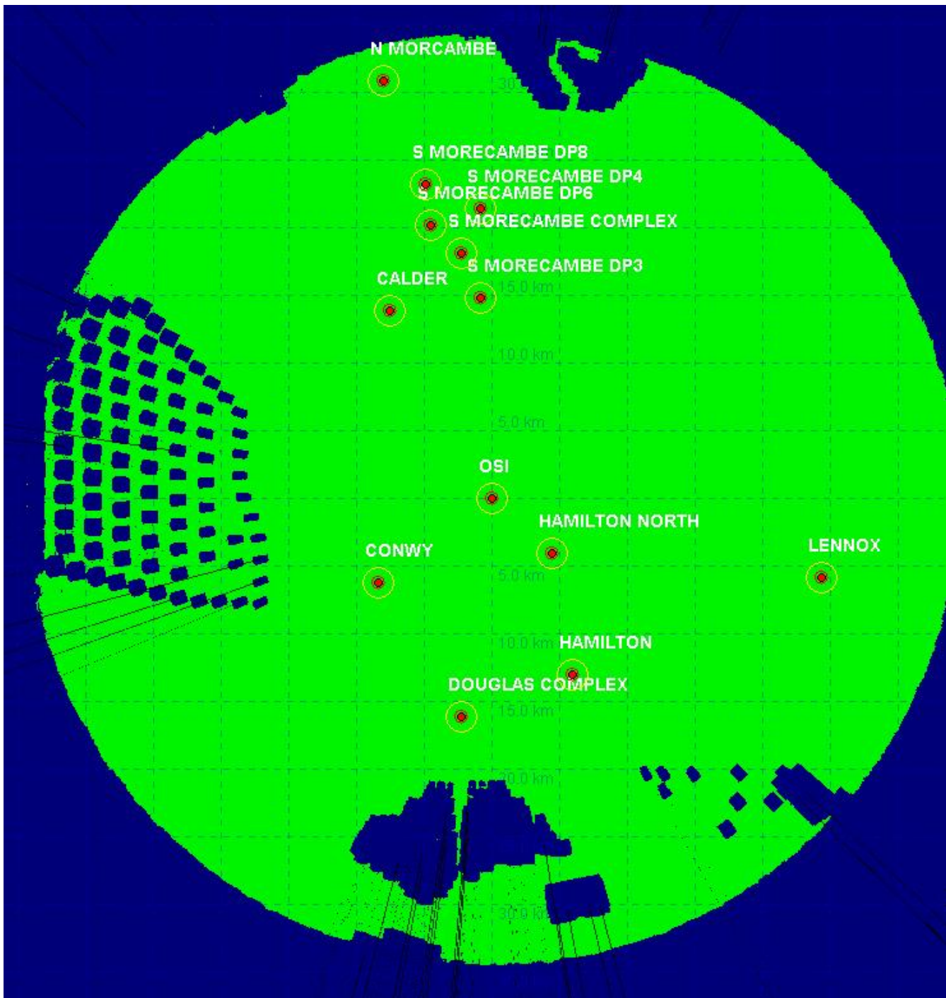
Figure 1.49: ENI Energy's OSI REWS detection plot showing loss regions for a 1,000 m 2 target.
